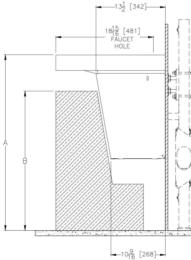
SIDE VIEW
